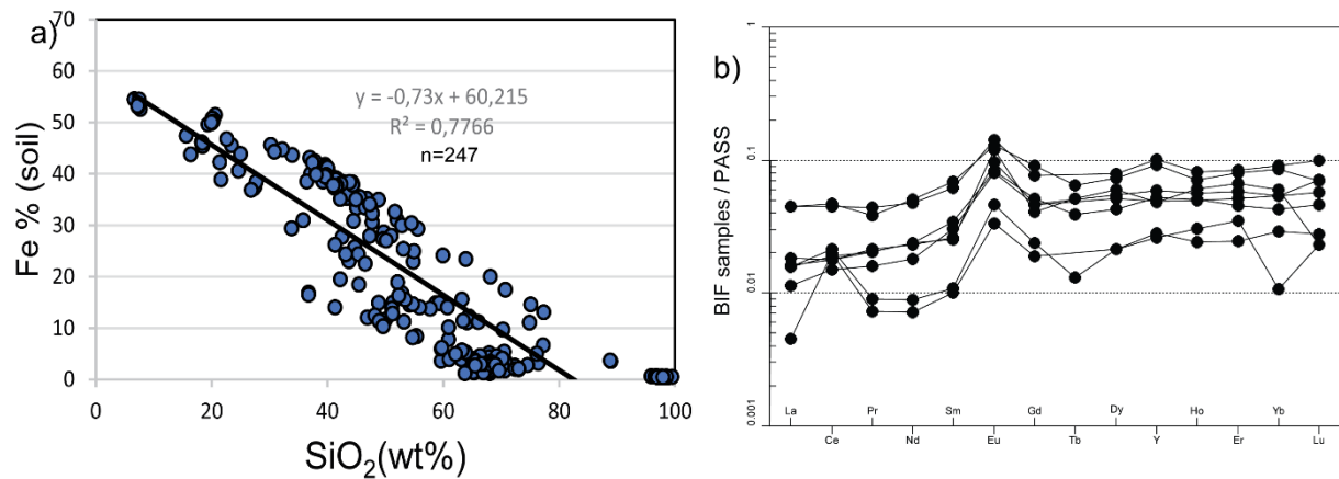
Fig.2. (a) Fe vs. SiO 2 in the soil samples of Sangmelima belt. (b) PAAS normalized fractionation diagrams for REE composition of BIFs in the SGB.
