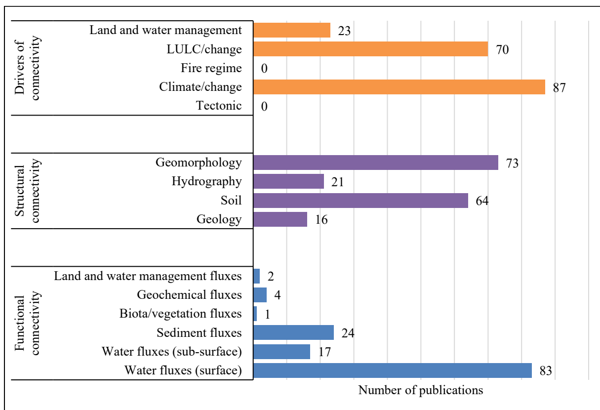
Figure 1 – Number of publications covering aspects of changing drivers of hydrologic connectivity, besides aspects of structural and functional connectivity, following the concepts proposed by Keesstra et al. (2018). One publication can cover multiple (sub)aspects.
