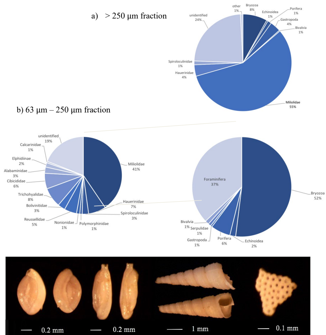
Figure 1: Relative contributions of the different classes of non-foraminiferal components and foraminiferal families in (a) the > 250 \mu\text{m} fraction and (b) the 63 \mu\text{m} – 250 \mu\text{m} fraction. c) from left to right: 2 miliolid specimens, 1 turrillid specimen, 1 bryozoan fragment.
