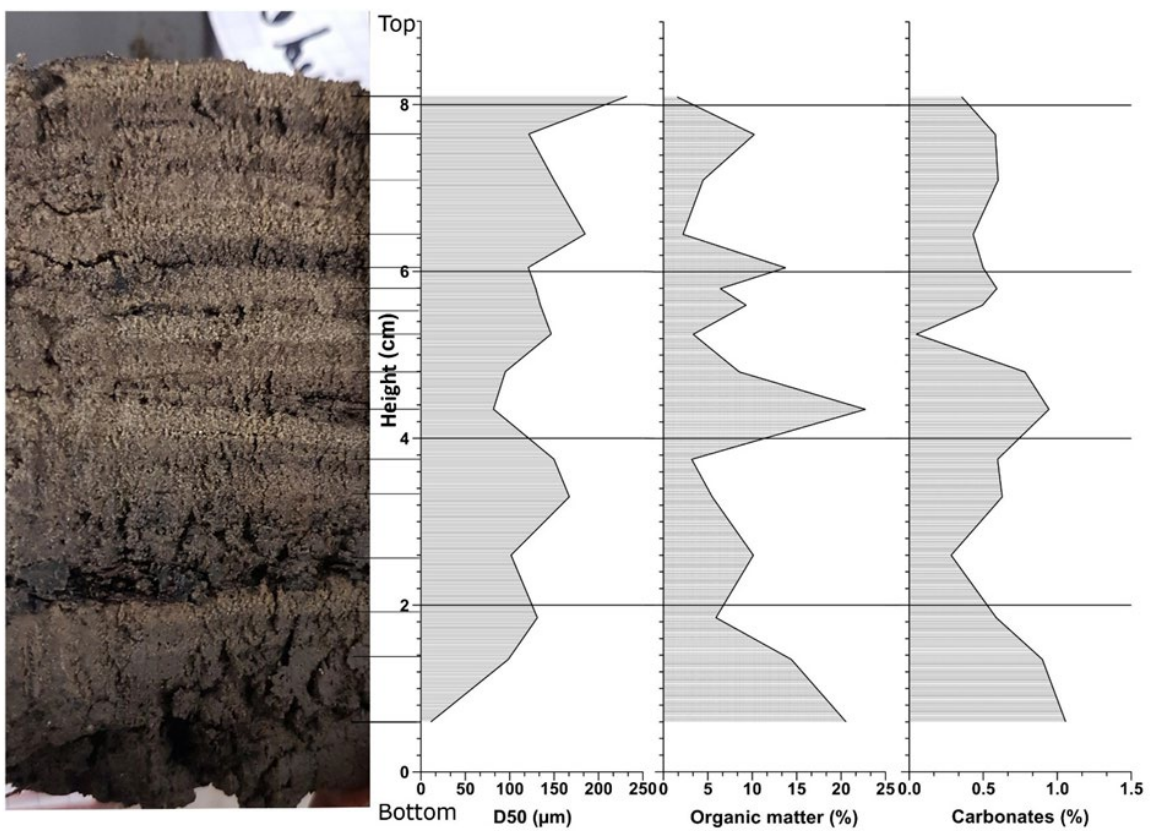
Fig 2: Sediment characterisation of the Draperie cave's deposit
