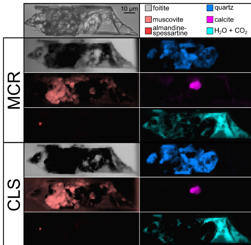
Figure 1. Raman mapping experiment of a crystalline melt inclusion in tourmaline from the Emmons Pegmatite. Phase identification is performed by spectra matching algorithms and the mapping data is resolved by both (1) Multivariate Curve Resolution Alternating Least Squares (MCR-ALS) and (2) Classical Least Squares (CLS) multivariate statistics.
