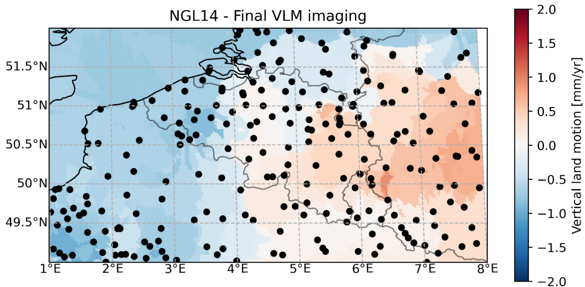
Figure 1 Imaging of the vertical land motion (VLM) over Belgium using a dense network of GNSS position time series computed by the Nevada Geodetic Laboratory.
