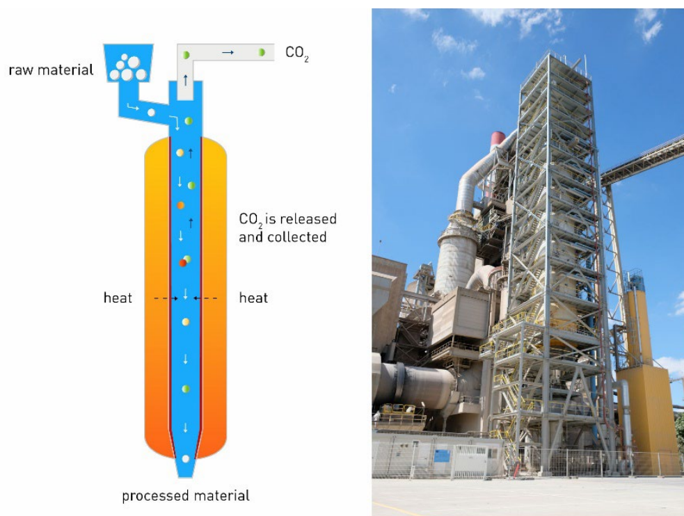
Figure 1. Left: schematic section of the LEILAC1 capture plant. Right: LEILAC1 capture plant at the Lixhe cement factory.
