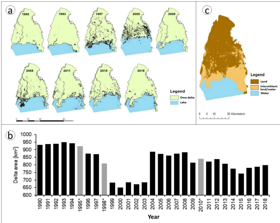
Figure 1 - Variation in the area of the Omo Delta for the period 1990-2018. (a) Extent of the area based on Landsat images and determined by a Random Forest classification; (b) Area of the delta for the dry season of each year between 1990 and 2018. Since there were no cloud free dry season images for the years 1995, 1998 and 2010, the delta area for these years was imputed using the mean of the three adjacent years. (c) Extent of the areas that was persistently either water or land, next to area which was intermittently either land or water.
