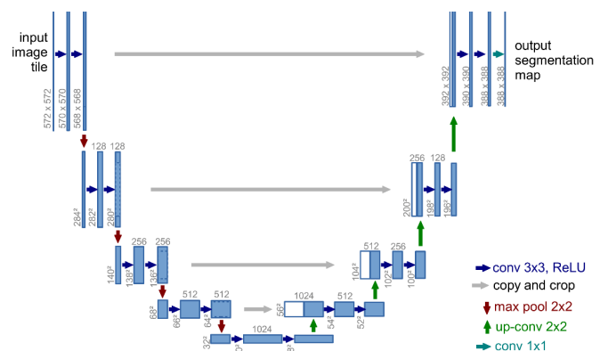
Figure 3: U-net architecture
